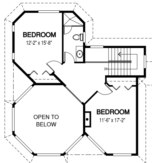
Upper Floor
