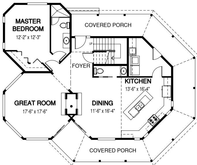
Main Floor
