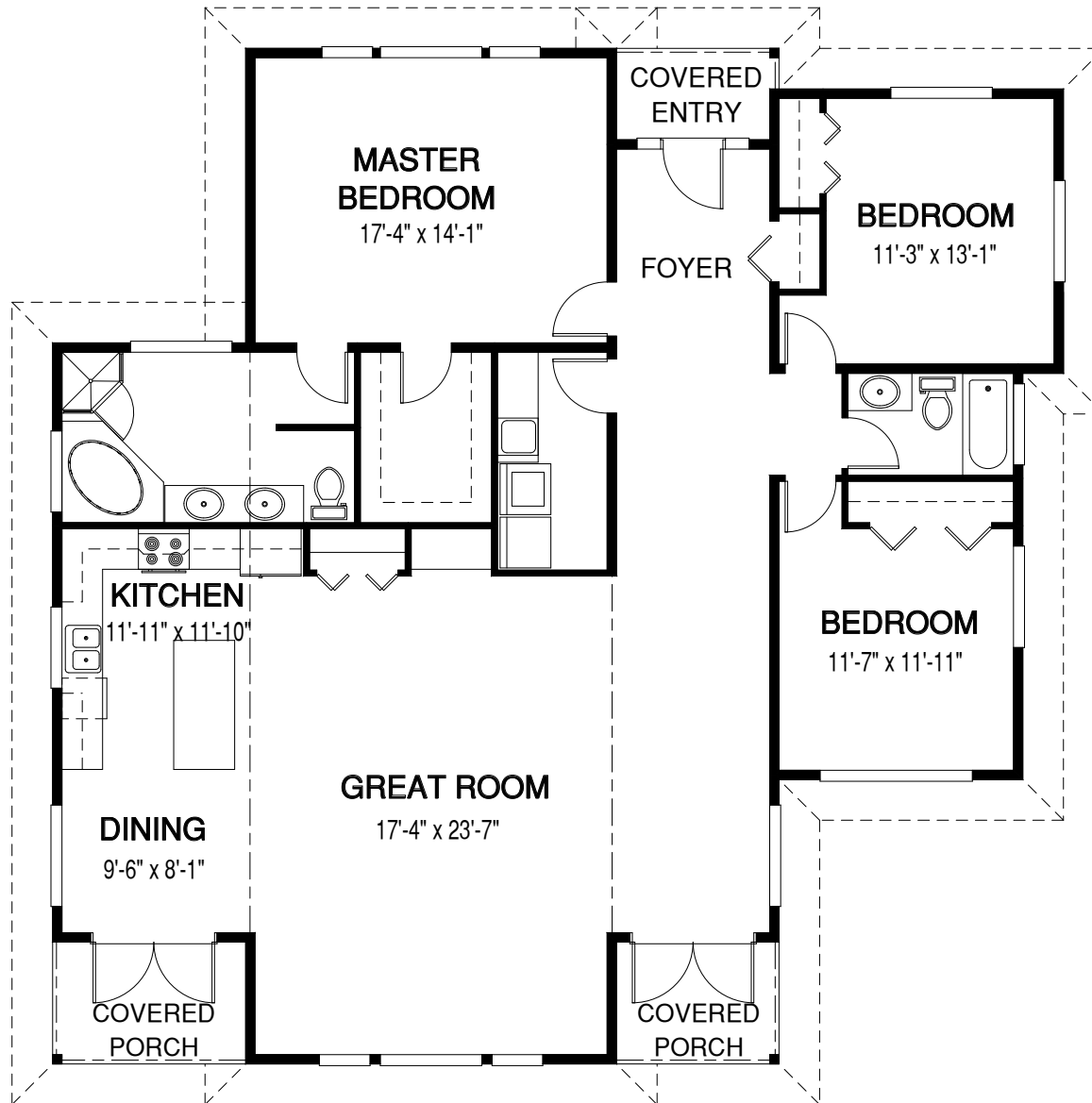
Main Floor
