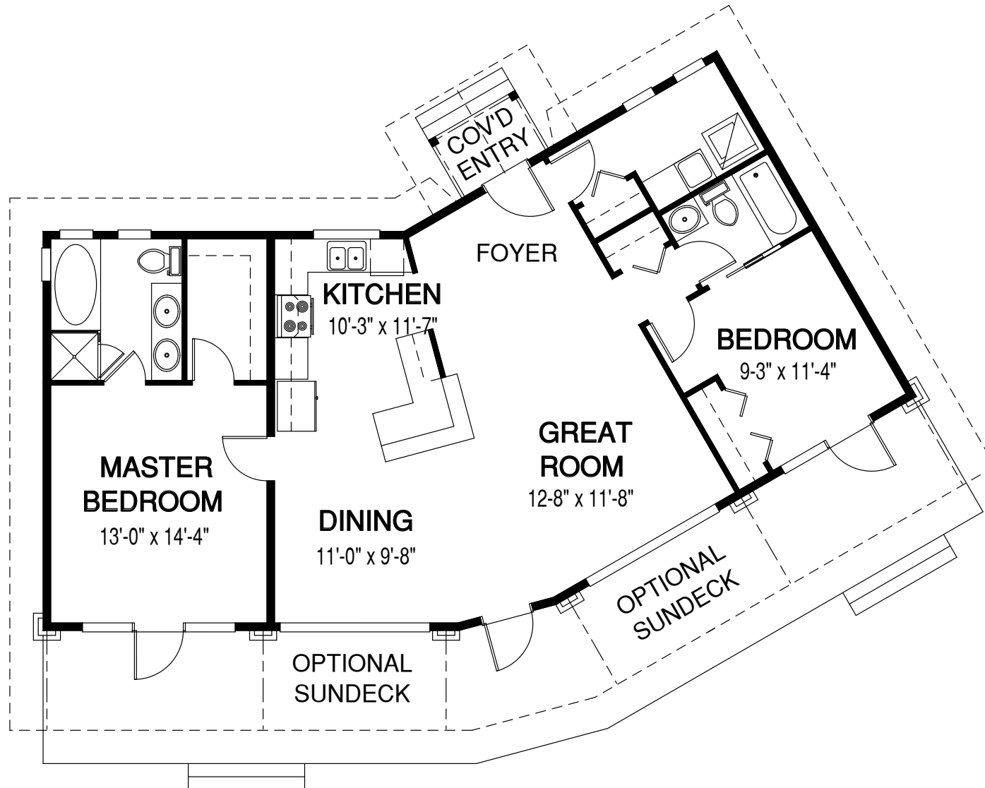
Main Floor
