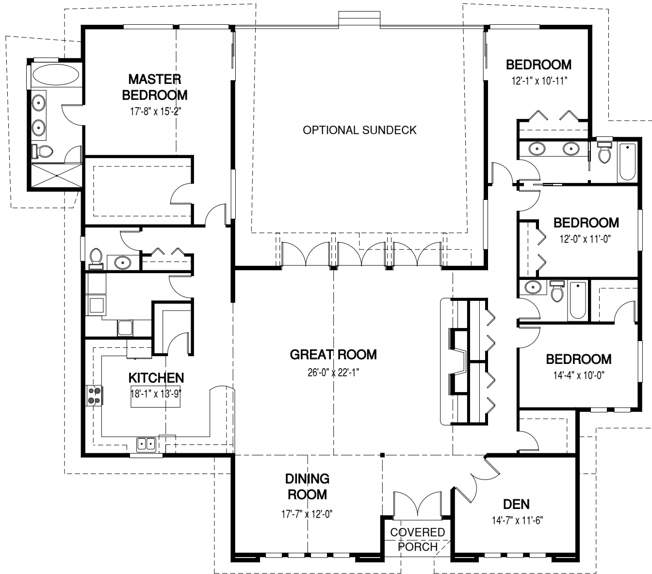
Main Floor
